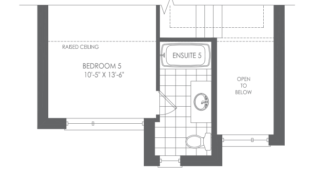
PARTIAL OPTIONAL THIRD FLOOR ELEV. B 5 BEDROOM PLAN
