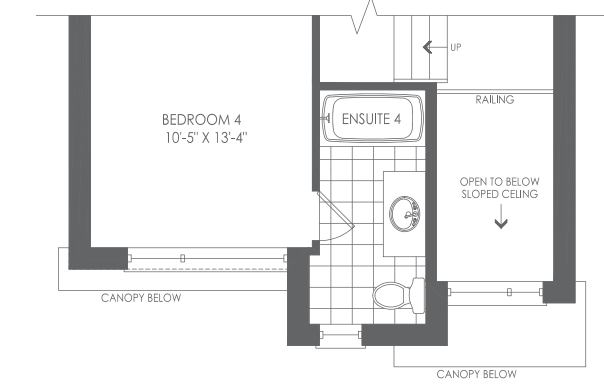
PARTIAL SECOND FLOOR ELEV. B
